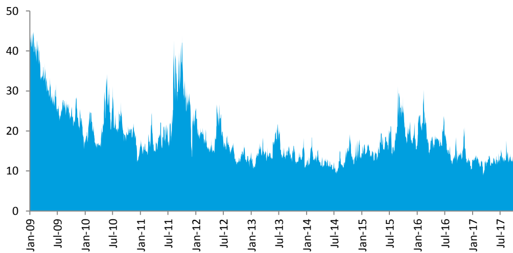
S&P/ASX 200 VIX
